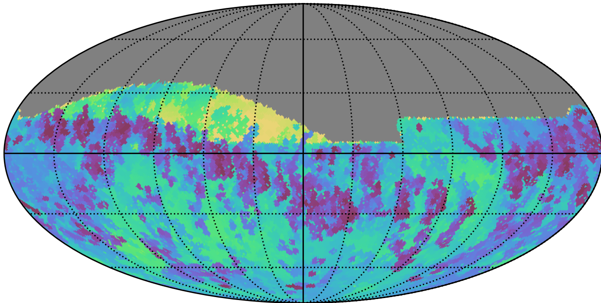
early_u_fpextra2.0_v3.4_10yrs Yr 1 all bands: Min skyBrightness
