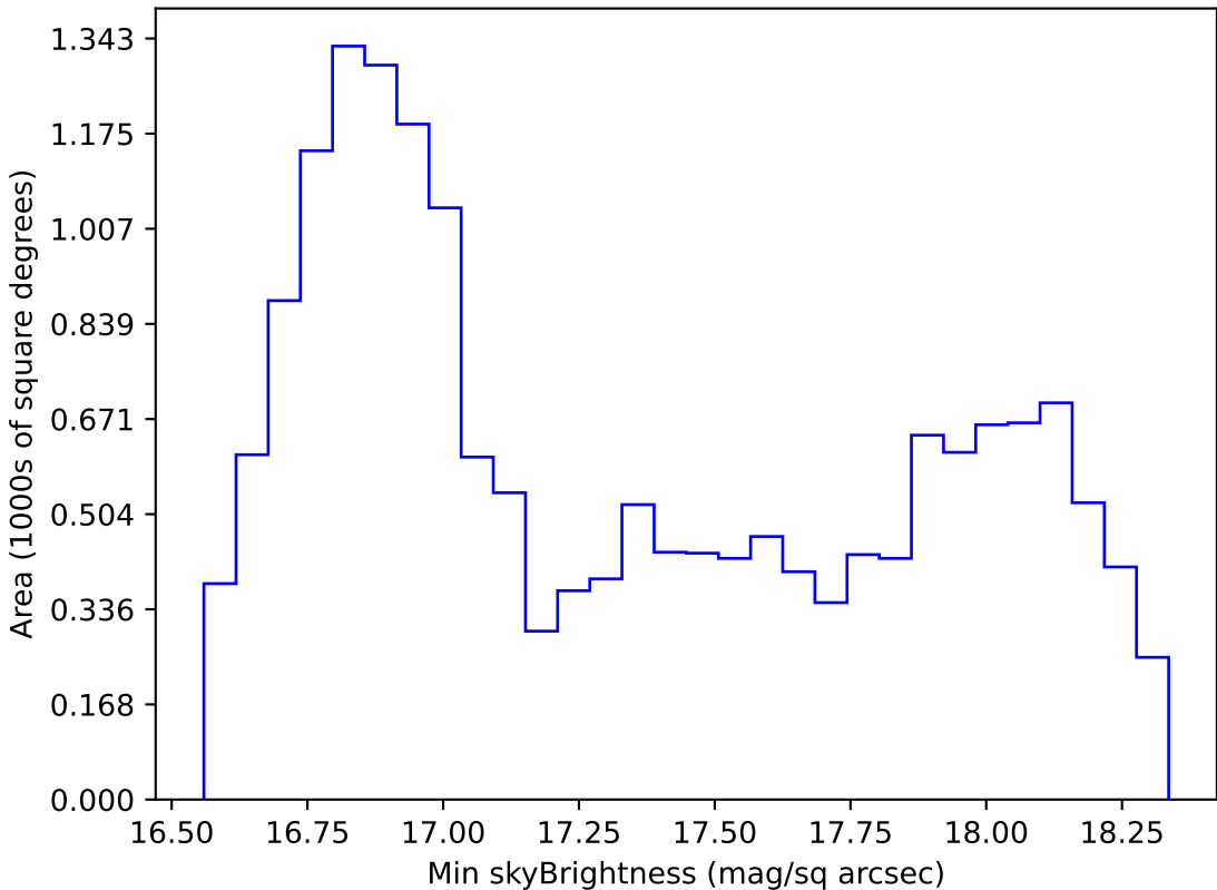
early_u_fpextra2.0_v3.4_10yrs WFD z band: Min skyBrightness
