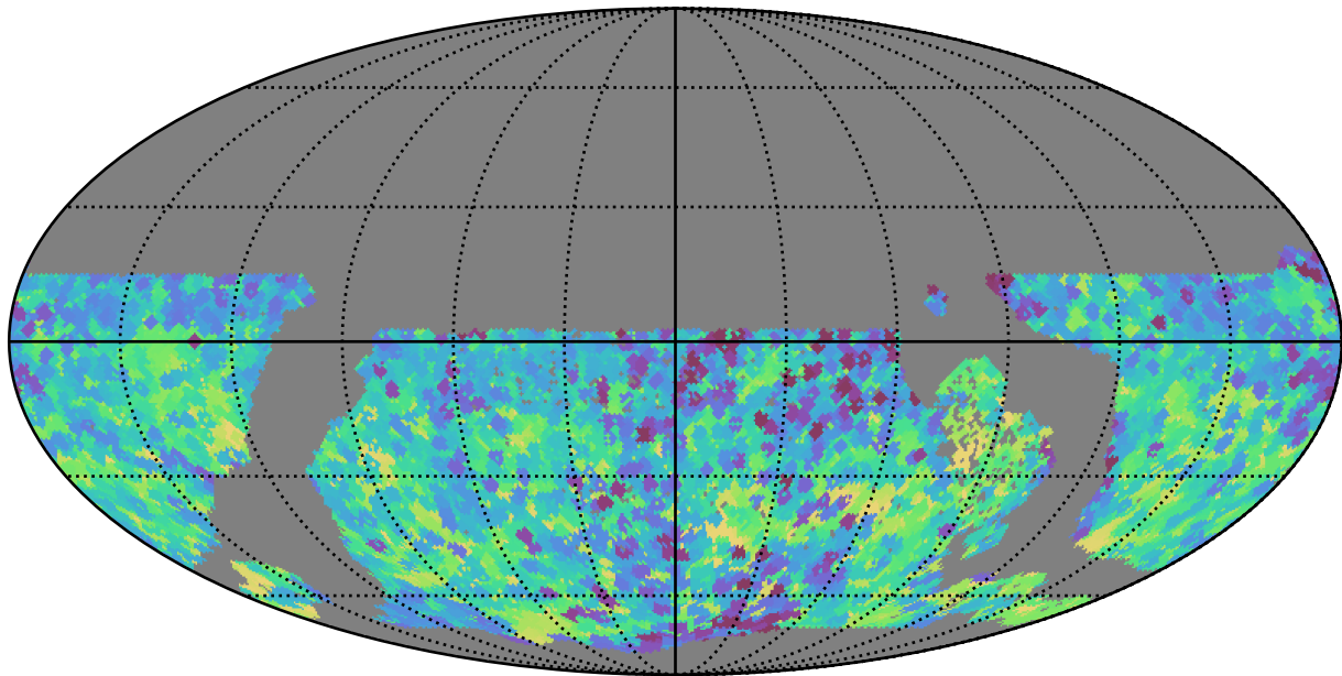
early_u_fpextra2.0_v3.4_10yrs WFD y band: Min skyBrightness
