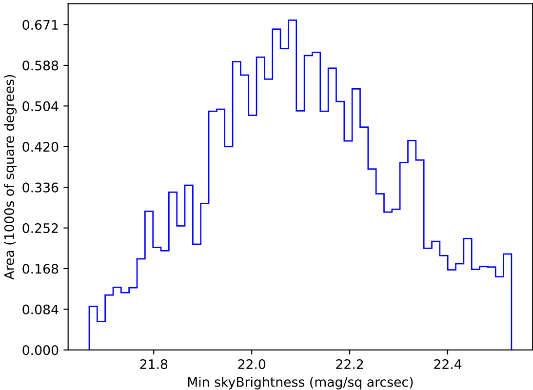
early_u_fpextra2.0_v3.4_10yrs WFD u band: Min skyBrightness
