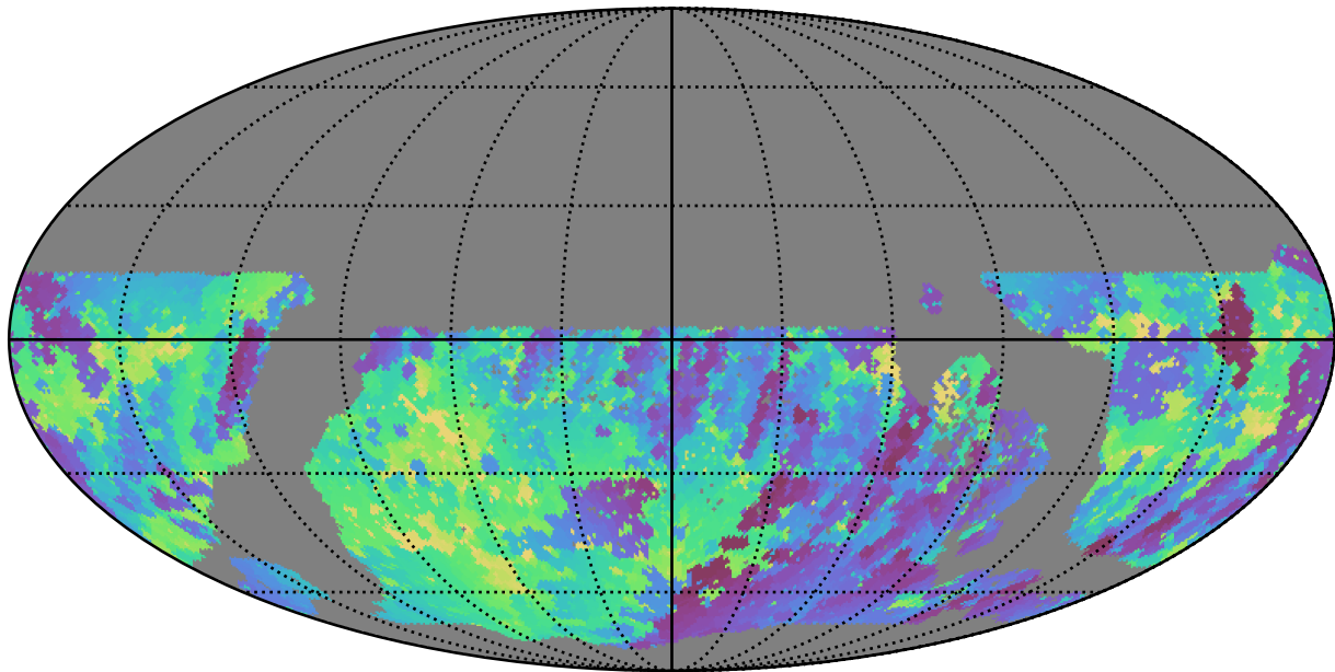
early_u_fpextra2.0_v3.4_10yrs WFD r band: Min skyBrightness
