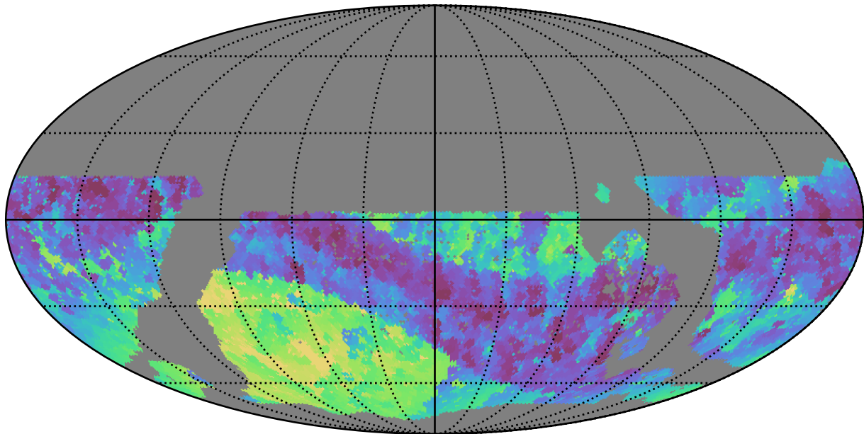
early_u_fpextra2.0_v3.4_10yrs WFD i band: Min skyBrightness
