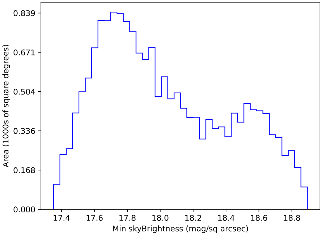
early_u_fpextra2.0_v3.4_10yrs WFD i band: Min skyBrightness
