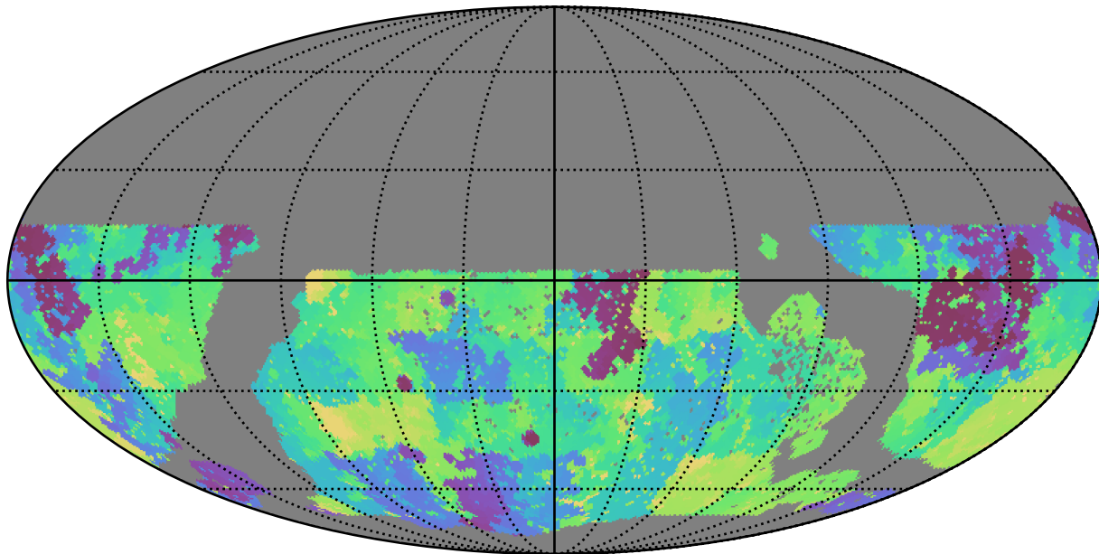
early_u_fpextra2.0_v3.4_10yrs WFD g band: Min skyBrightness
