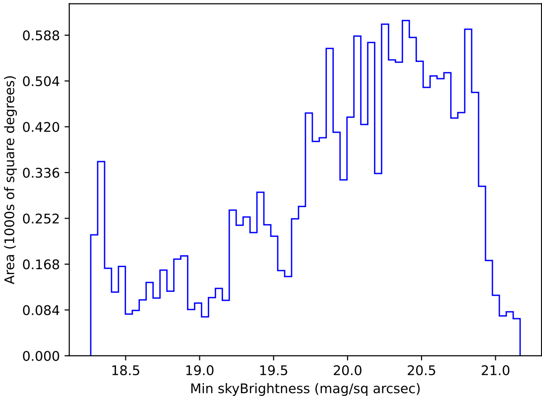
early_u_fpextra2.0_v3.4_10yrs WFD g band: Min skyBrightness
