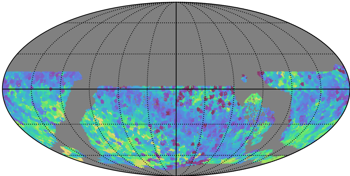
early_u_fpextra2.0_v3.4_10yrs WFD all bands: Min skyBrightness
