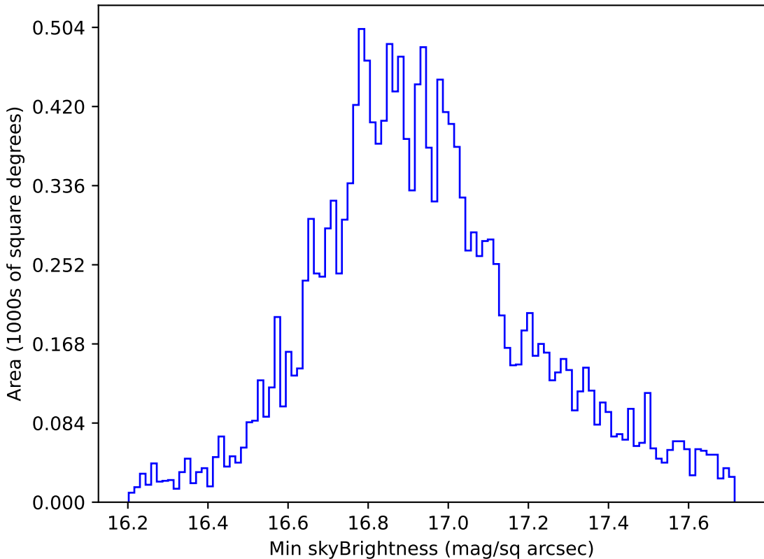
early_u_fpextra2.0_v3.4_10yrs WFD all bands: Min skyBrightness
