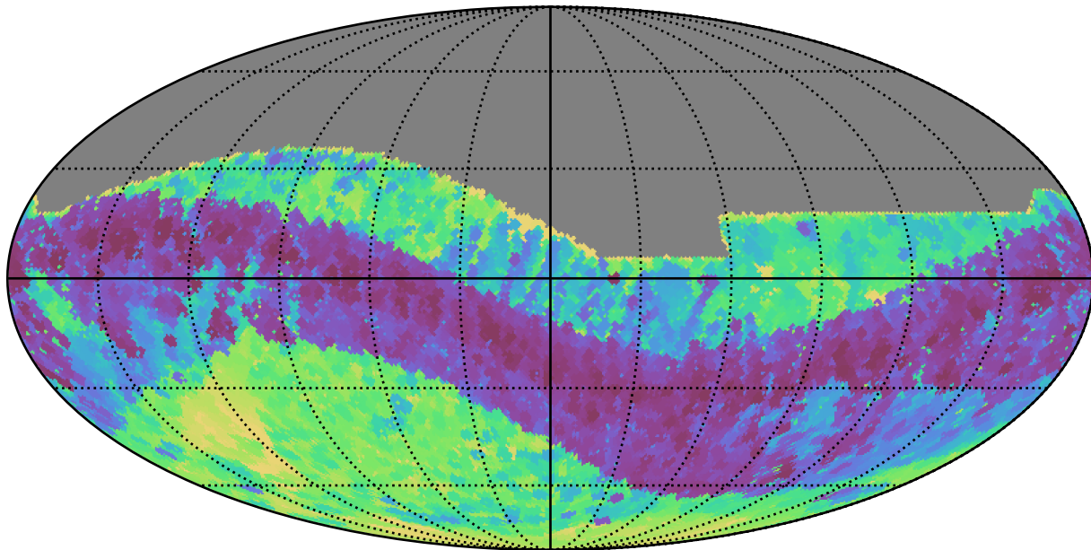
early_u_fpextra2.0_v3.4_10yrs All sky z band: Min skyBrightness
