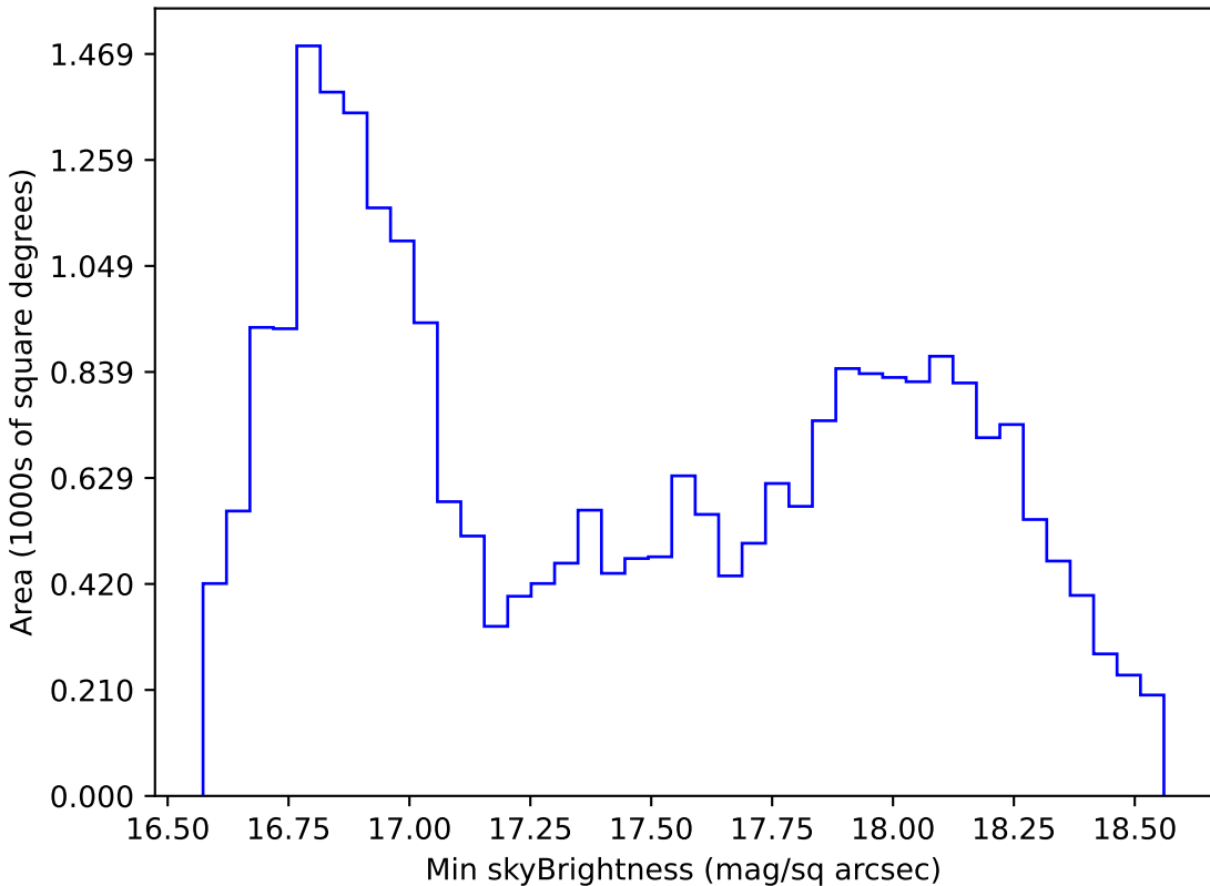
early_u_fpextra2.0_v3.4_10yrs All sky z band: Min skyBrightness
