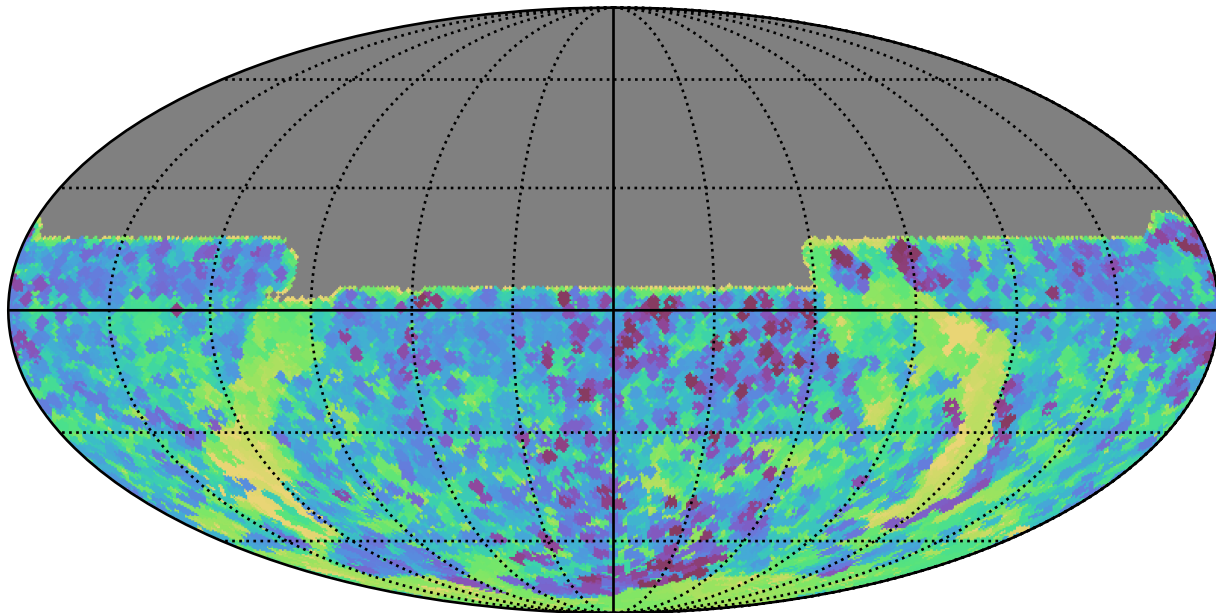
early_u_fpextra2.0_v3.4_10yrs All sky y band: Min skyBrightness
