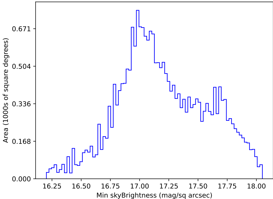
early_u_fpextra2.0_v3.4_10yrs All sky y band: Min skyBrightness
