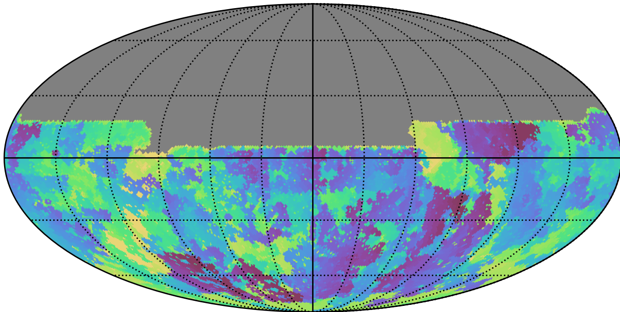
early_u_fpextra2.0_v3.4_10yrs All sky u band: Min skyBrightness
