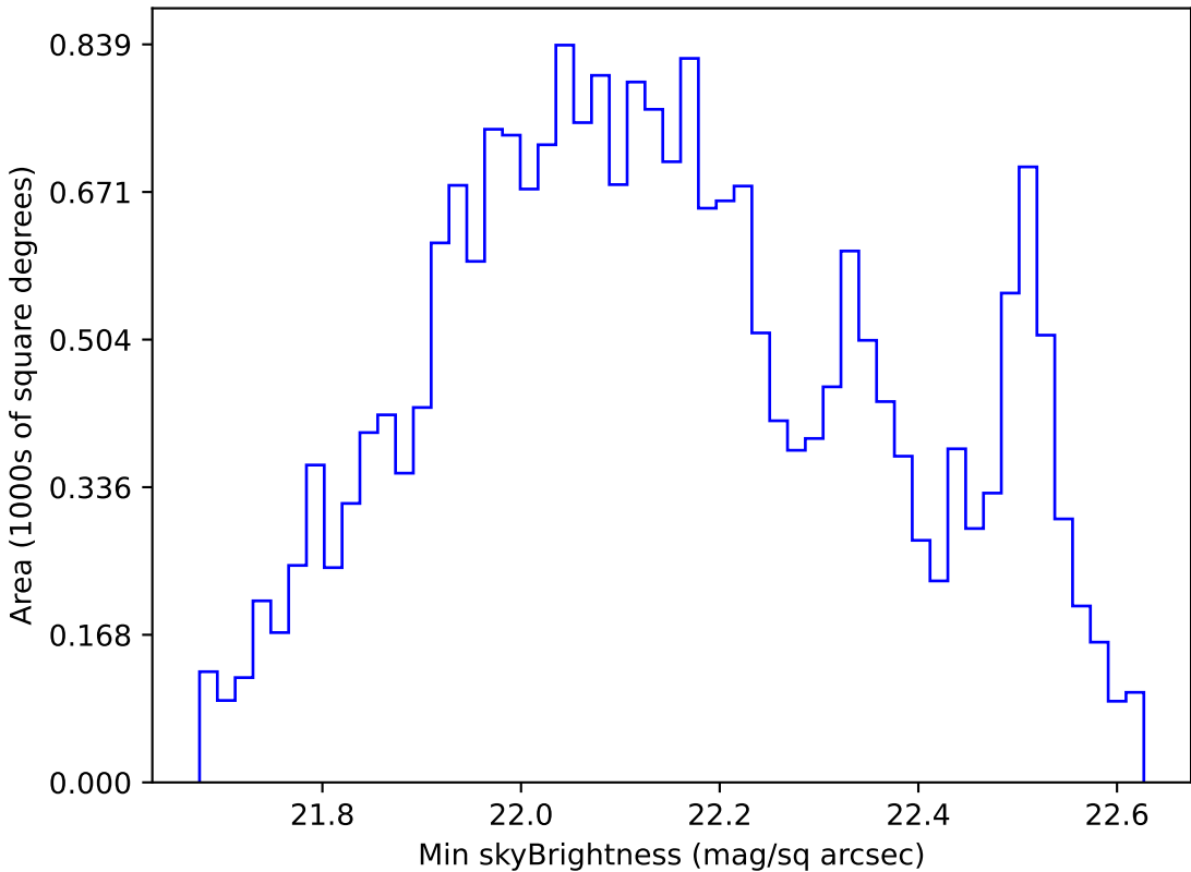
early_u_fpextra2.0_v3.4_10yrs All sky u band: Min skyBrightness
