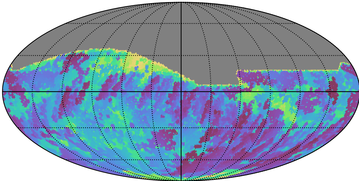
early_u_fpextra2.0_v3.4_10yrs All sky r band: Min skyBrightness
