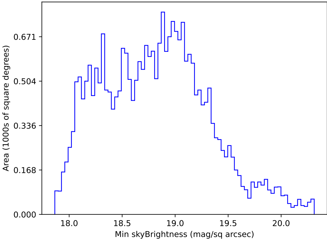
early_u_fpextra2.0_v3.4_10yrs All sky r band: Min skyBrightness
