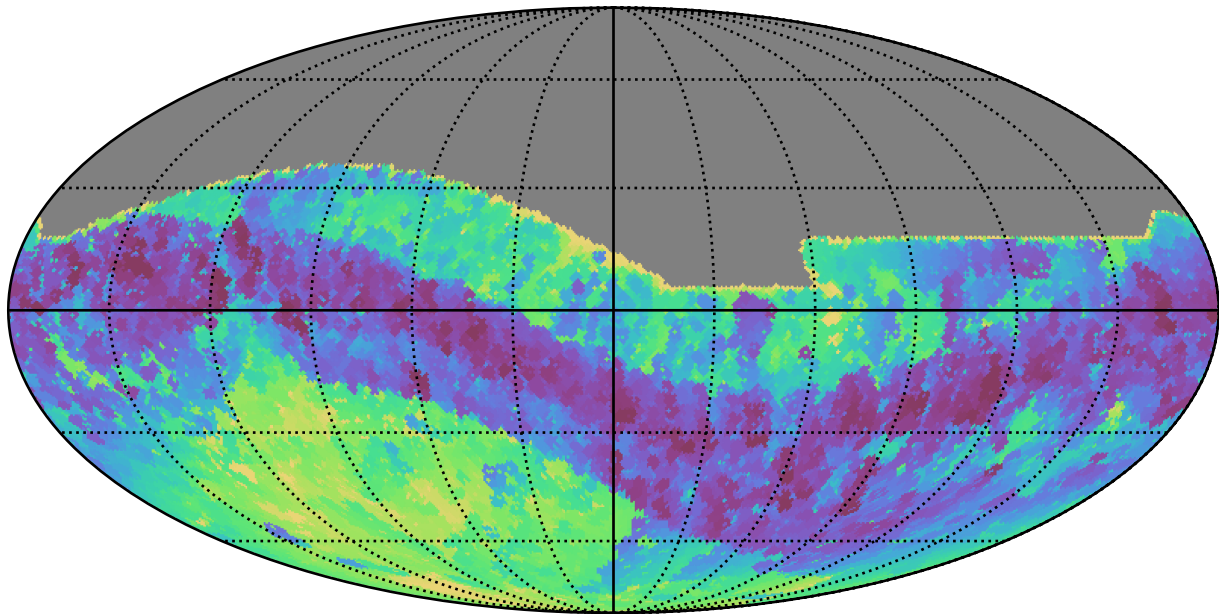
early_u_fpextra2.0_v3.4_10yrs All sky i band: Min skyBrightness
