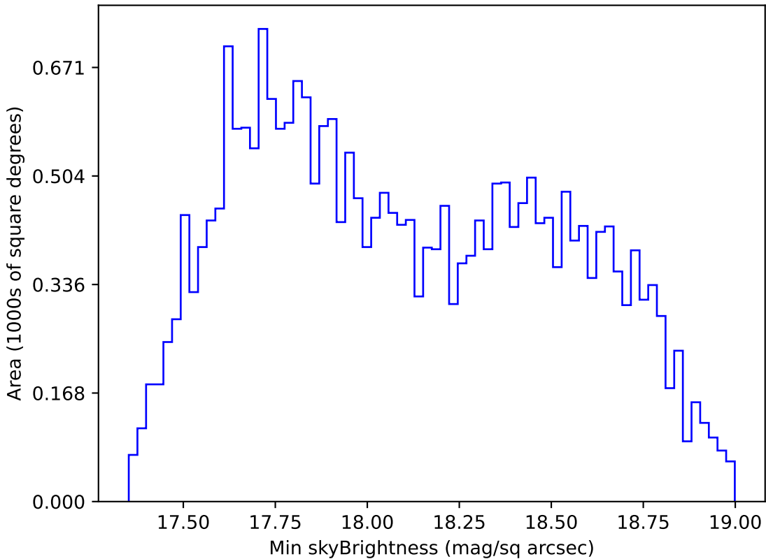
early_u_fpextra2.0_v3.4_10yrs All sky i band: Min skyBrightness
