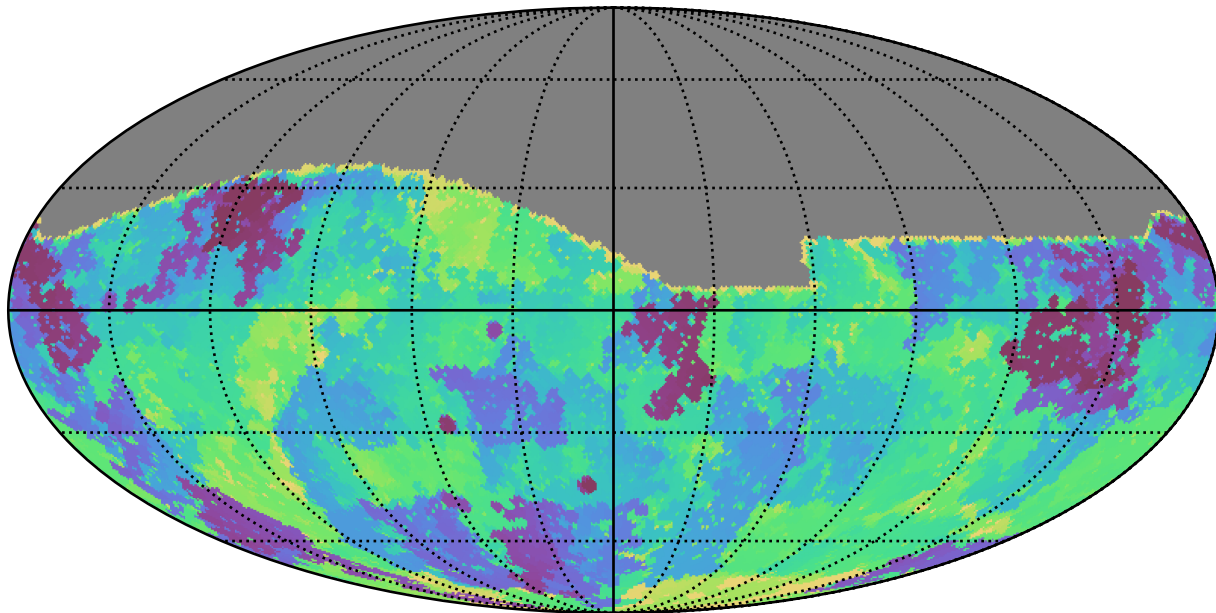
early_u_fpextra2.0_v3.4_10yrs All sky g band: Min skyBrightness
