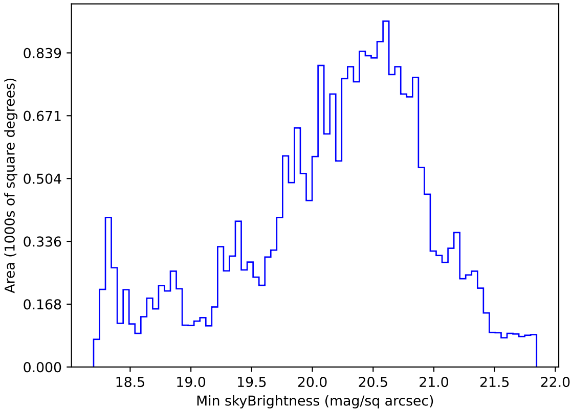
early_u_fpextra2.0_v3.4_10yrs All sky g band: Min skyBrightness
