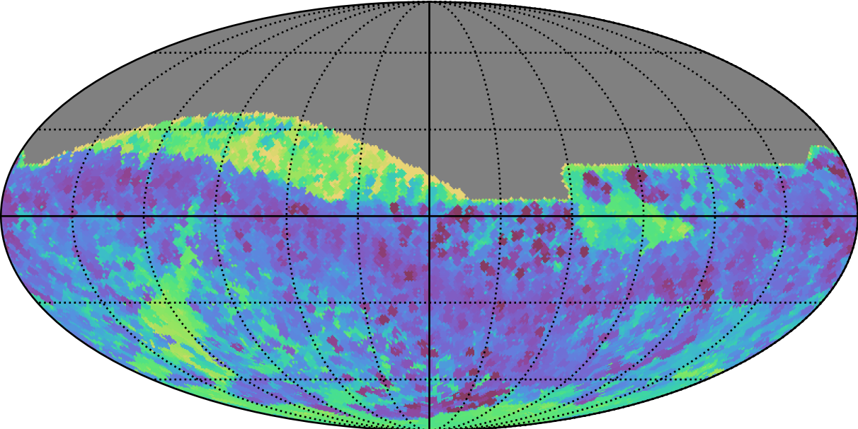
early_u_fpextra2.0_v3.4_10yrs All sky all bands: Min skyBrightness
