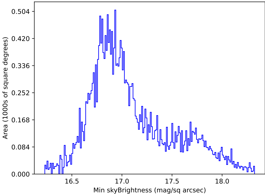
early_u_fpextra2.0_v3.4_10yrs All sky all bands: Min skyBrightness
