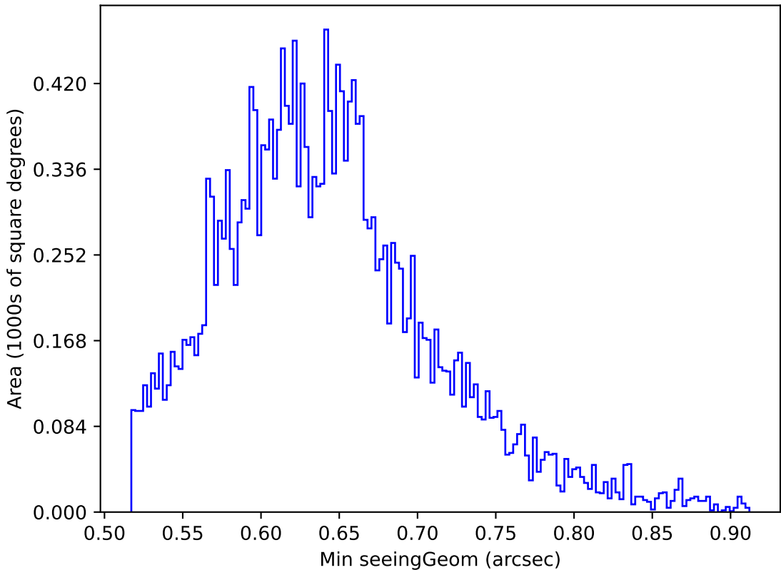
early_u_fpextra2.0_v3.4_10yrs Yr 1 y band: Min seeingGeom
