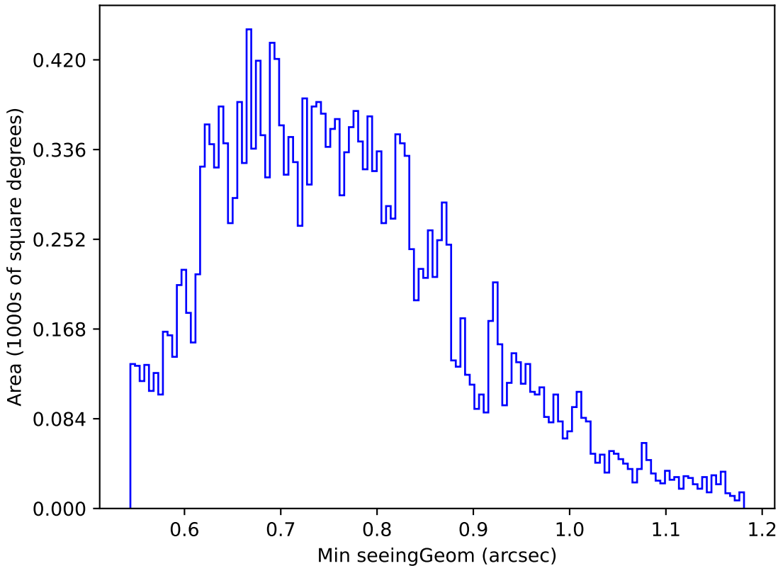
early_u_fpextra2.0_v3.4_10yrs Yr 1 u band: Min seeingGeom
