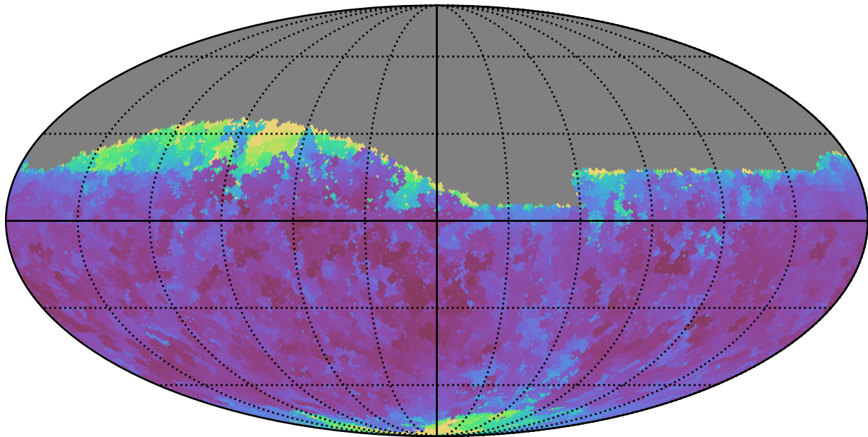
early_u_fpextra2.0_v3.4_10yrs Yr 1 r band: Min seeingGeom
