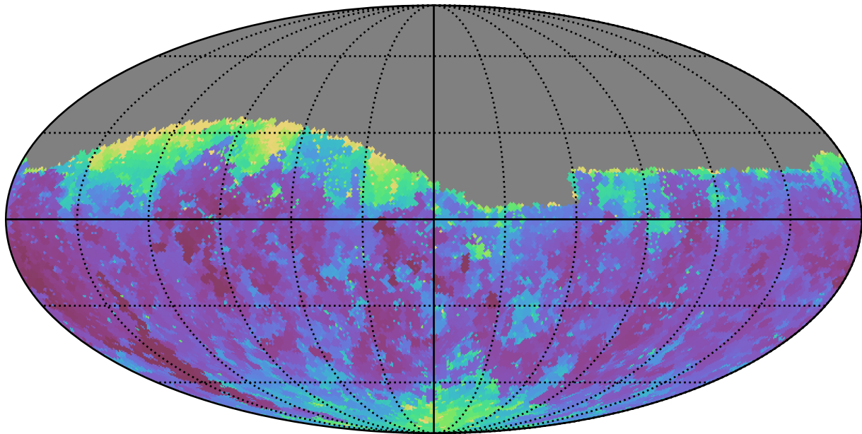
early_u_fpextra2.0_v3.4_10yrs Yr 1 g band: Min seeingGeom
