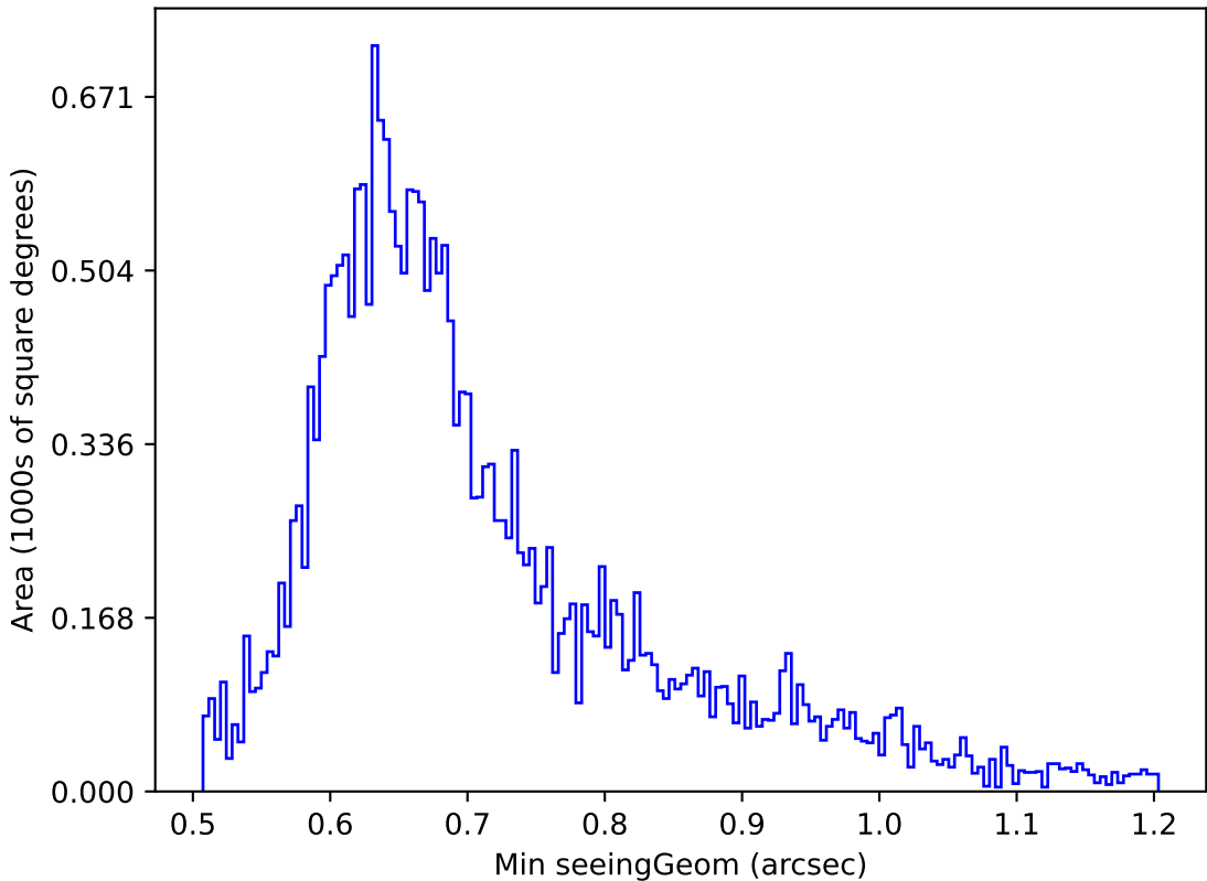
early_u_fpextra2.0_v3.4_10yrs Yr 1 g band: Min seeingGeom
