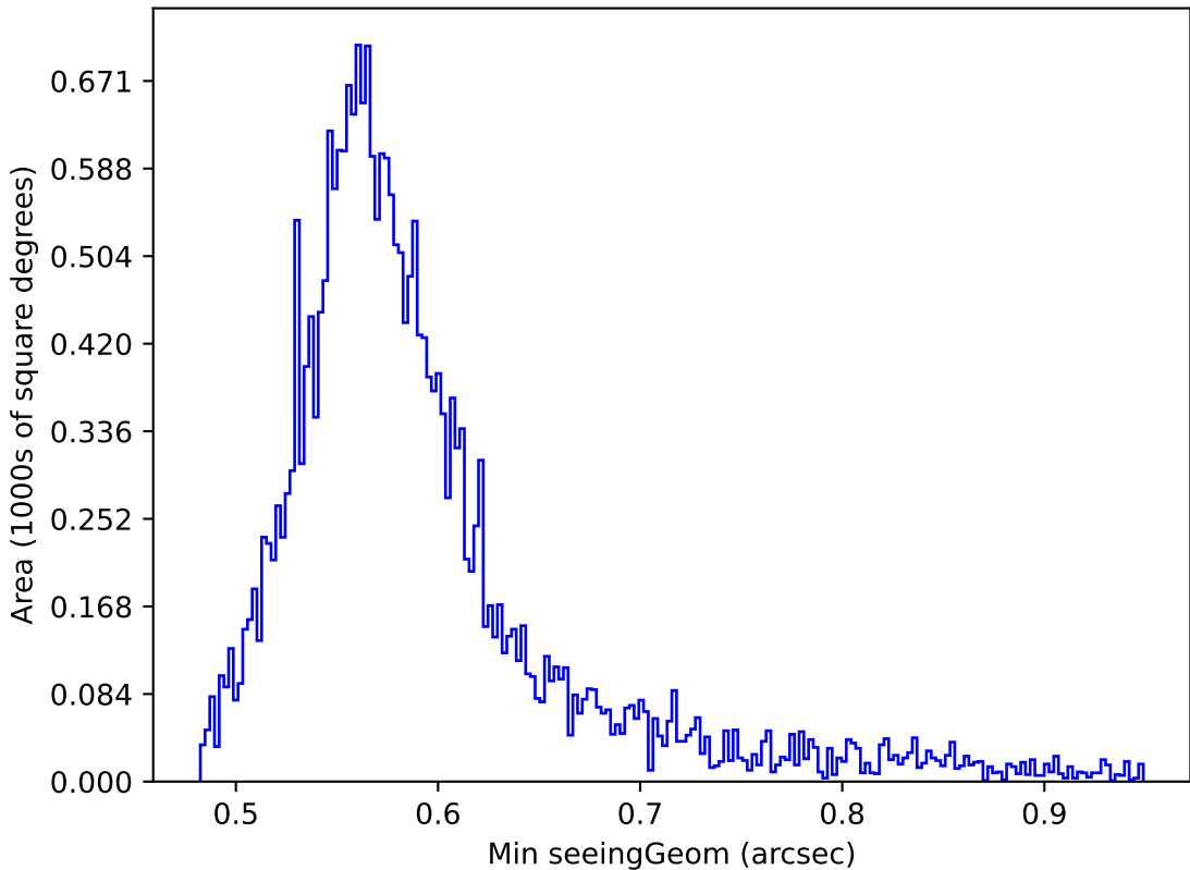
early_u_fpextra2.0_v3.4_10yrs Yr 1 all bands: Min seeingGeom
