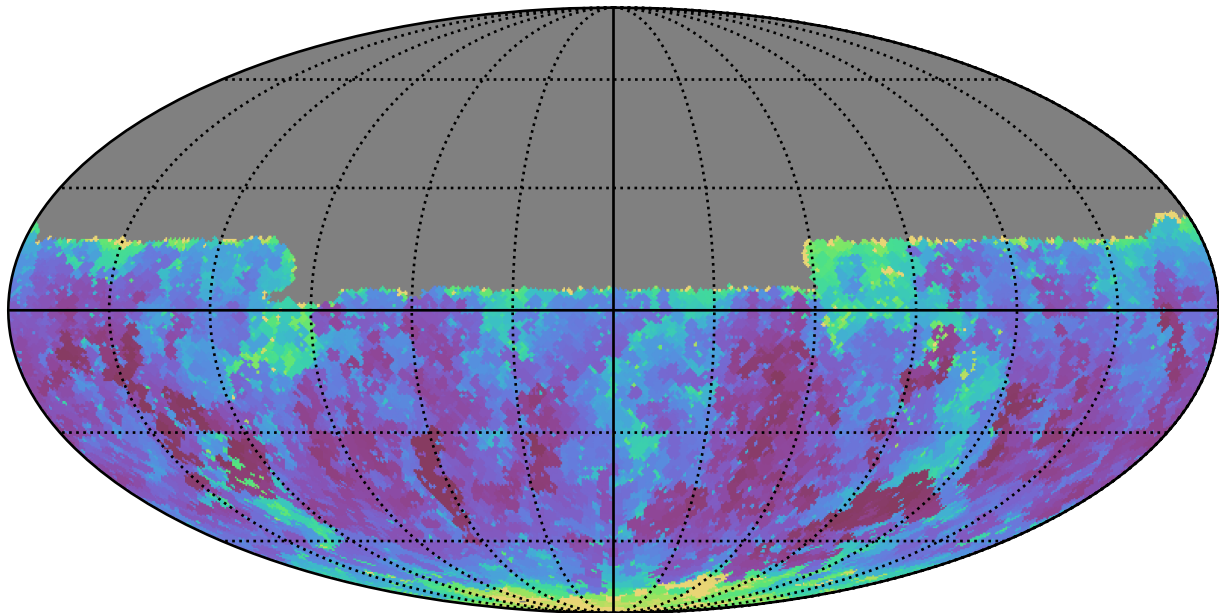
early_u_fpextra2.0_v3.4_10yrs Yr 1 y band: Min seeingEff
