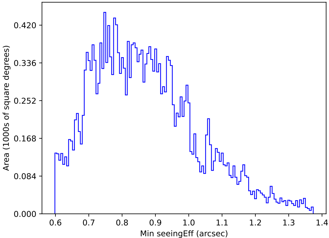
early_u_fpextra2.0_v3.4_10yrs Yr 1 u band: Min seeingEff
