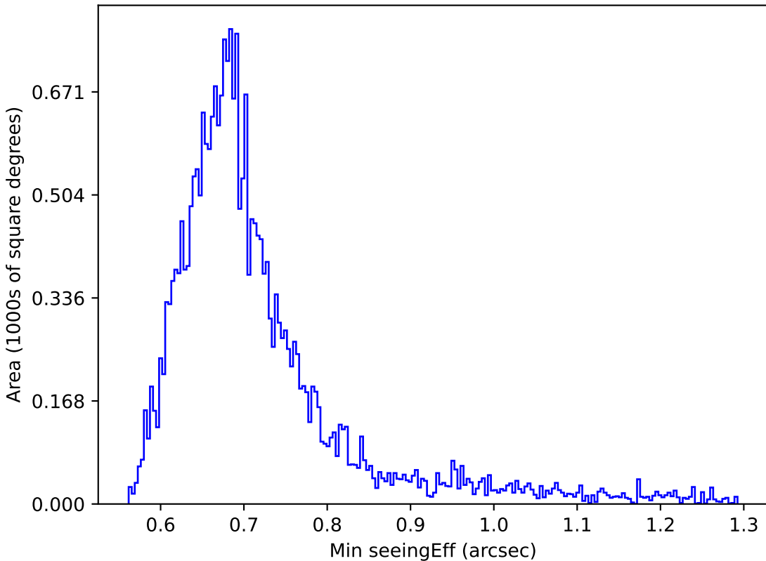
early_u_fpextra2.0_v3.4_10yrs Yr 1 r band: Min seeingEff
