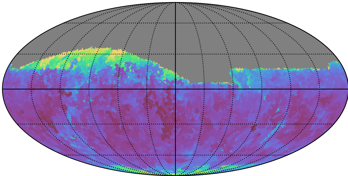
early_u_fpextra2.0_v3.4_10yrs Yr 1 i band: Min seeingEff
