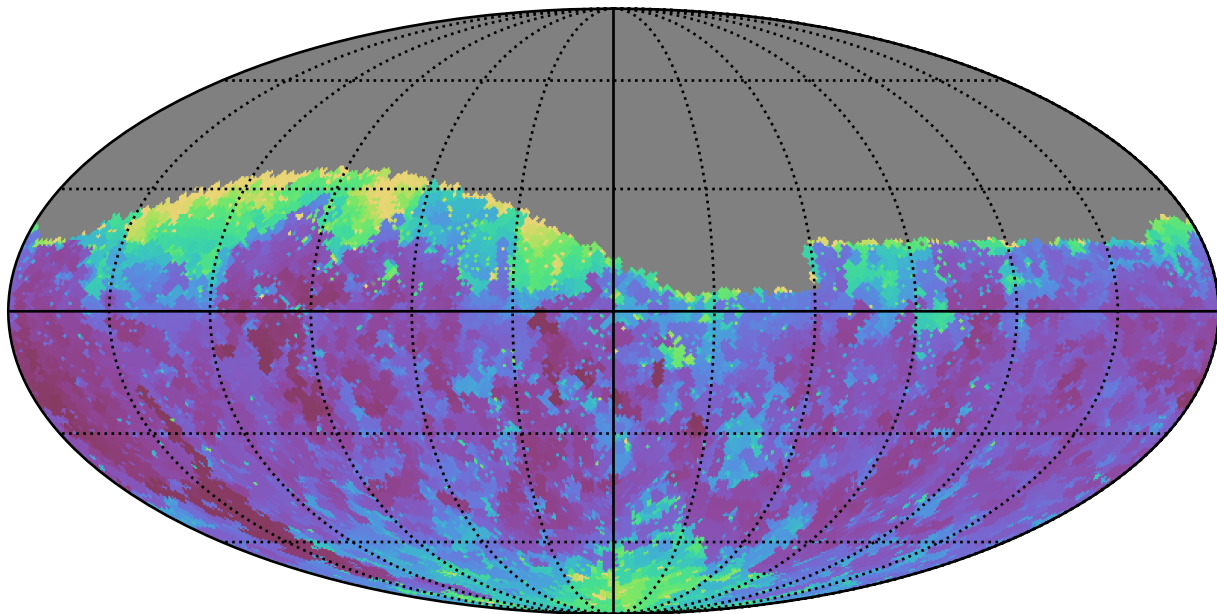
early_u_fpextra2.0_v3.4_10yrs Yr 1 g band: Min seeingEff
