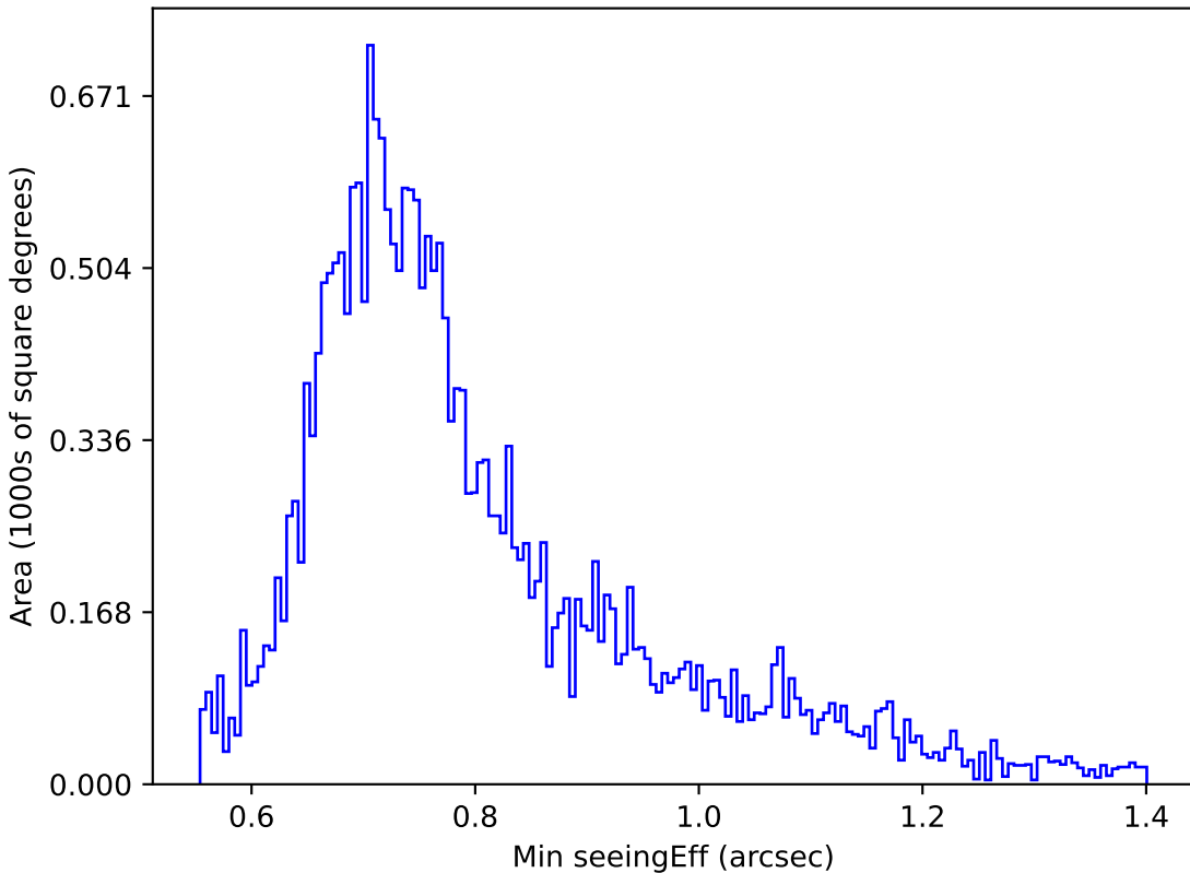
early_u_fpextra2.0_v3.4_10yrs Yr 1 g band: Min seeingEff
