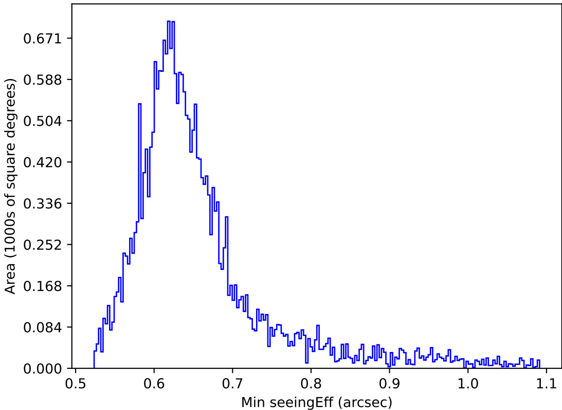
early_u_fpextra2.0_v3.4_10yrs Yr 1 all bands: Min seeingEff
