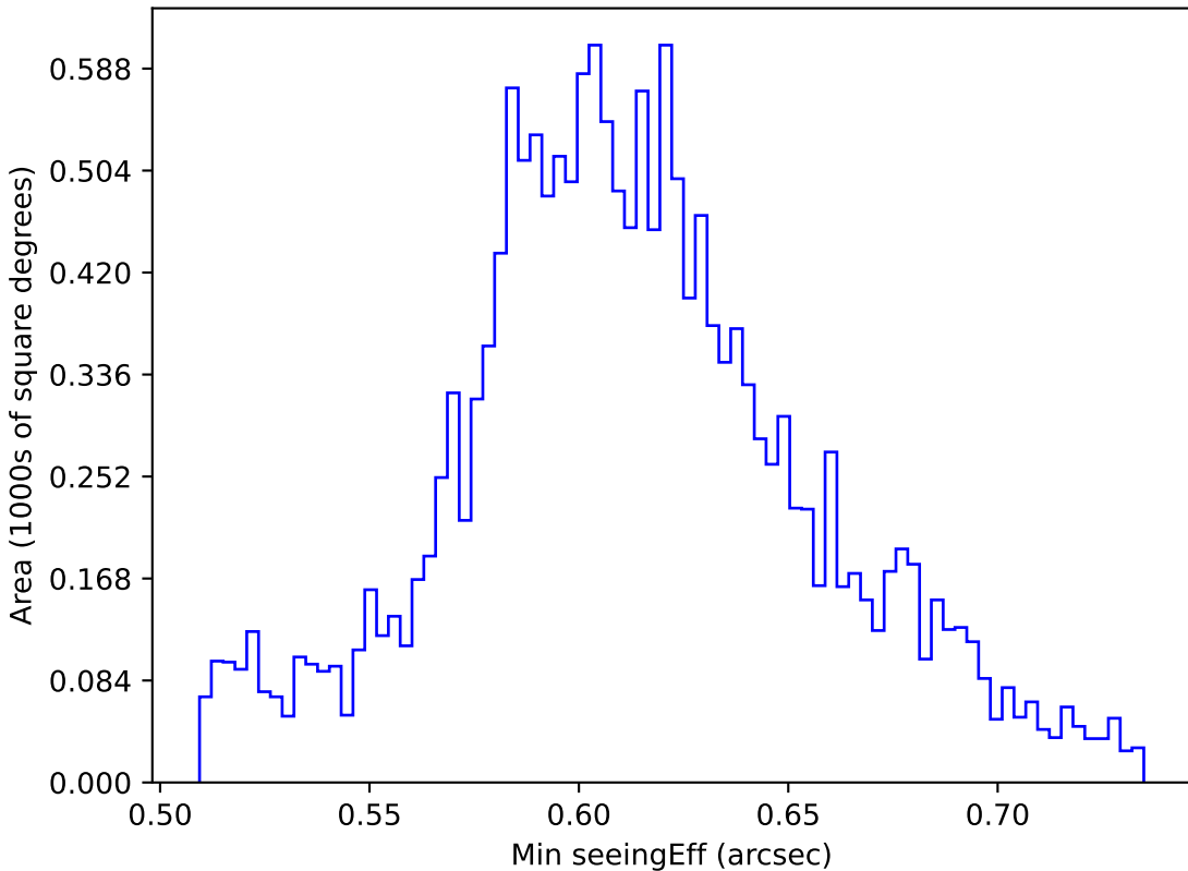
early_u_fpextra2.0_v3.4_10yrs WFD z band: Min seeingEff
