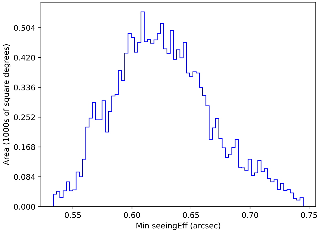
early_u_fpextra2.0_v3.4_10yrs WFD y band: Min seeingEff
