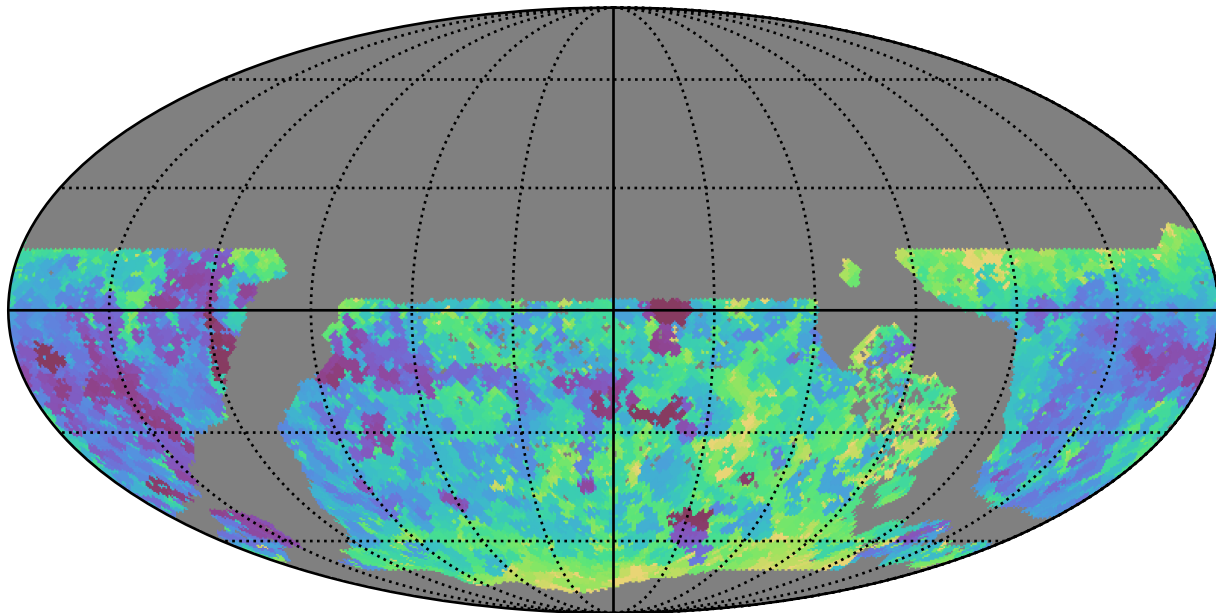
early_u_fpextra2.0_v3.4_10yrs WFD u band: Min seeingEff
