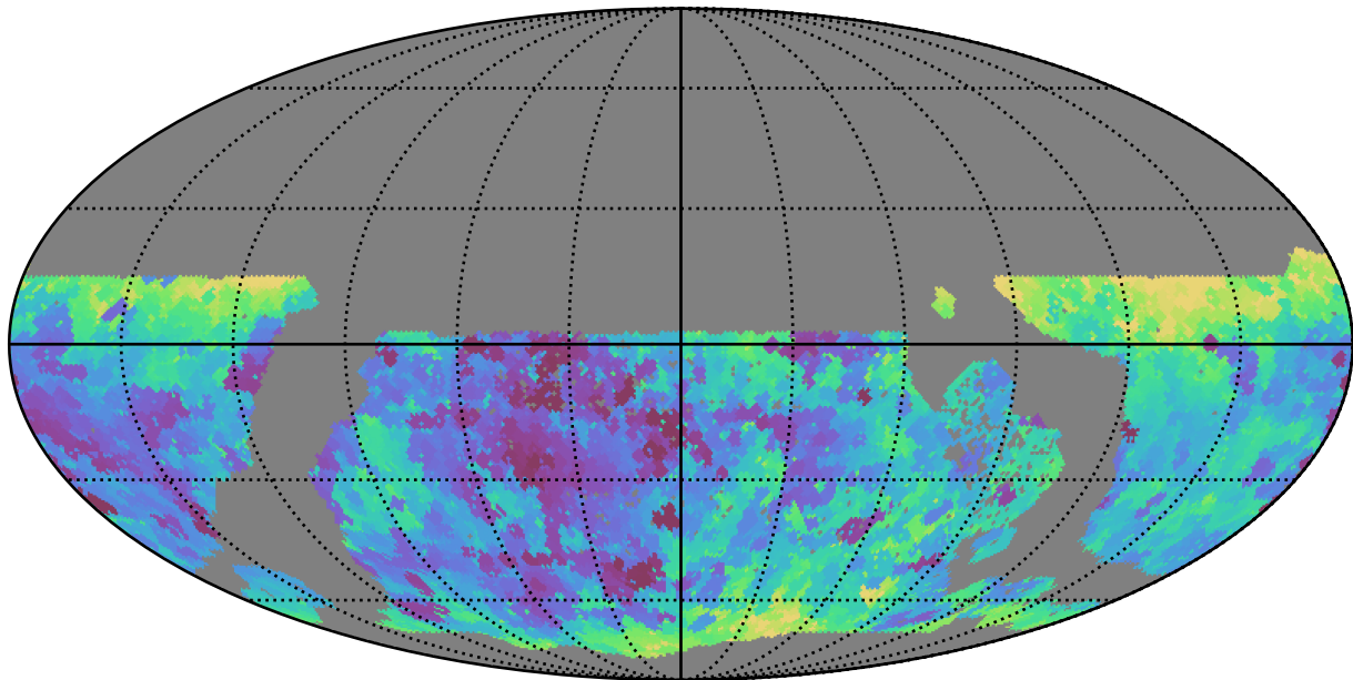
early_u_fpextra2.0_v3.4_10yrs WFD r band: Min seeingEff
