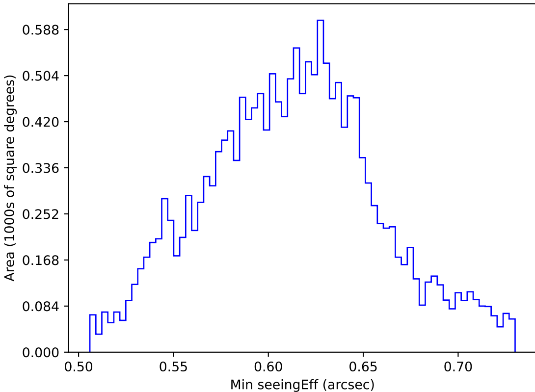
early_u_fpextra2.0_v3.4_10yrs WFD r band: Min seeingEff
