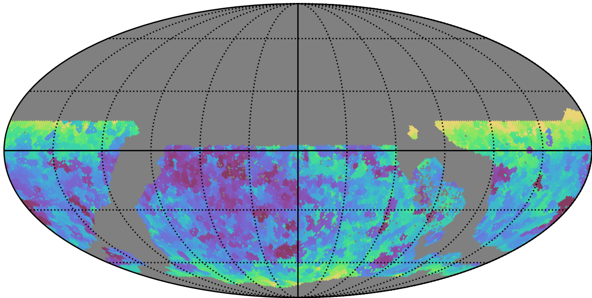
early_u_fpextra2.0_v3.4_10yrs WFD all bands: Min seeingEff
