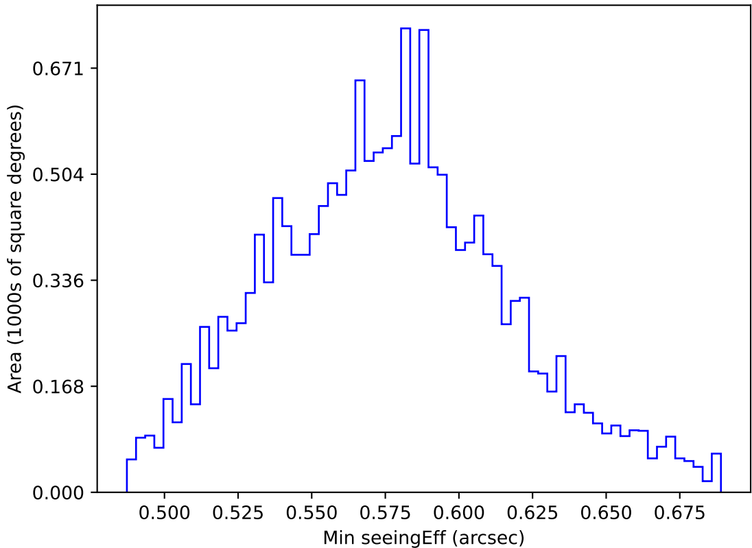
early_u_fpextra2.0_v3.4_10yrs WFD all bands: Min seeingEff
