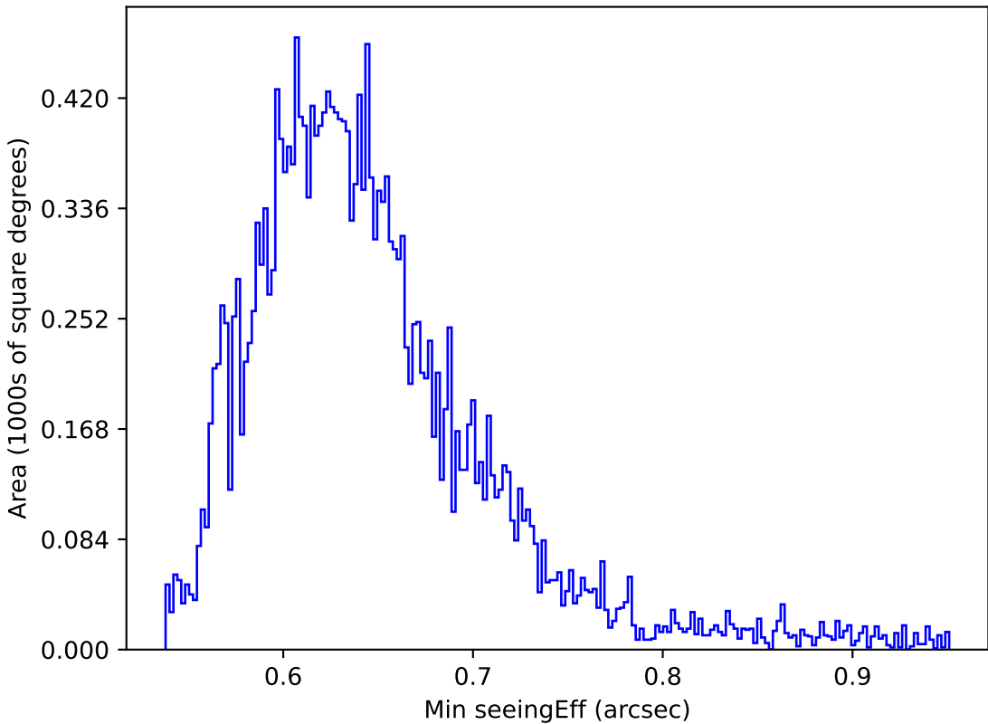
early_u_fpextra2.0_v3.4_10yrs All sky y band: Min seeingEff
