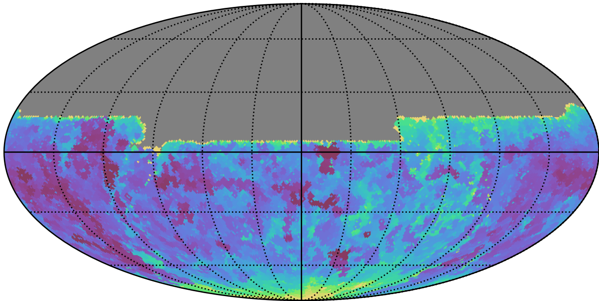
early_u_fpextra2.0_v3.4_10yrs All sky u band: Min seeingEff
