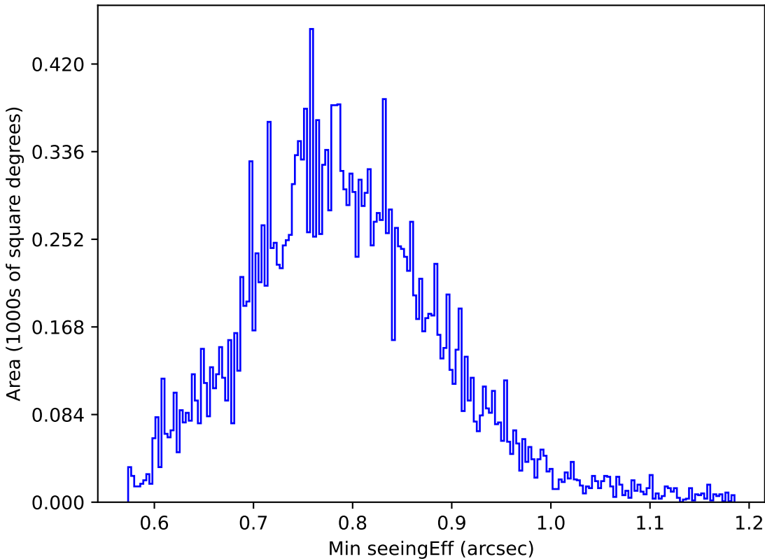
early_u_fpextra2.0_v3.4_10yrs All sky u band: Min seeingEff
