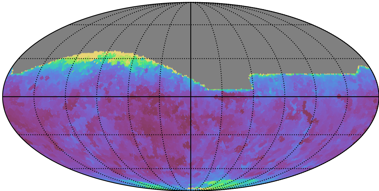
early_u_fpextra2.0_v3.4_10yrs All sky r band: Min seeingEff
