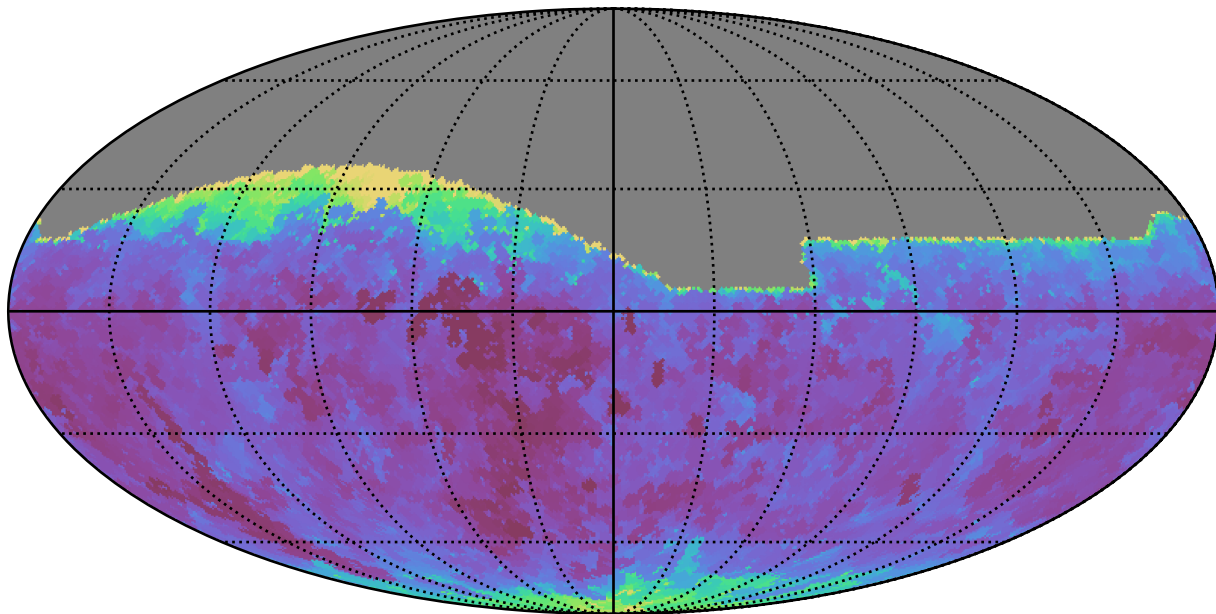
early_u_fpextra2.0_v3.4_10yrs All sky g band: Min seeingEff
